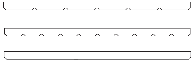
Cross-section of Troldtekt v-line 1way 6, v-line 1way 10 and v-line 1way blank. Panel size: 25 x 600 x 1200 mm.
